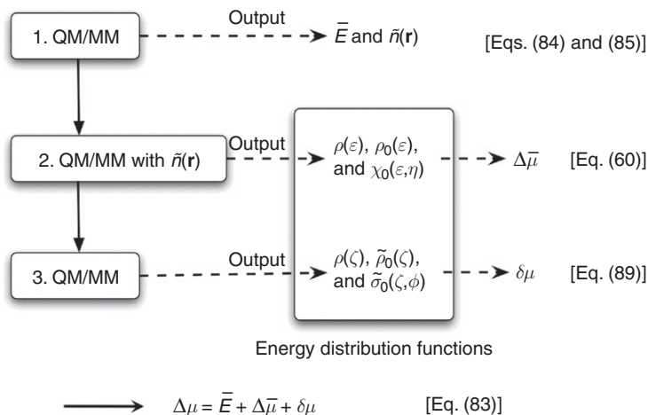
Figure 9.10 Flow chart for the procedure to compute solvation free energy by means of the QM/MM-ER approach. See the text for the detailed description for the energy distribution functions.
