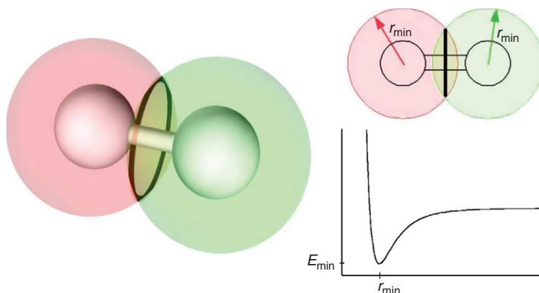
Figure 7.7 Application of standard MM potentials (e.g., Lennard-Jones 6–12 plus Coulomb potential) to \text{Hg}_2^{2+} predicts the favored ligand position at the intersection of the spheres with a radius r_{\min} . Data obtained from experiments and the QMCF simulation indicate that these positions are unfavored, however.
