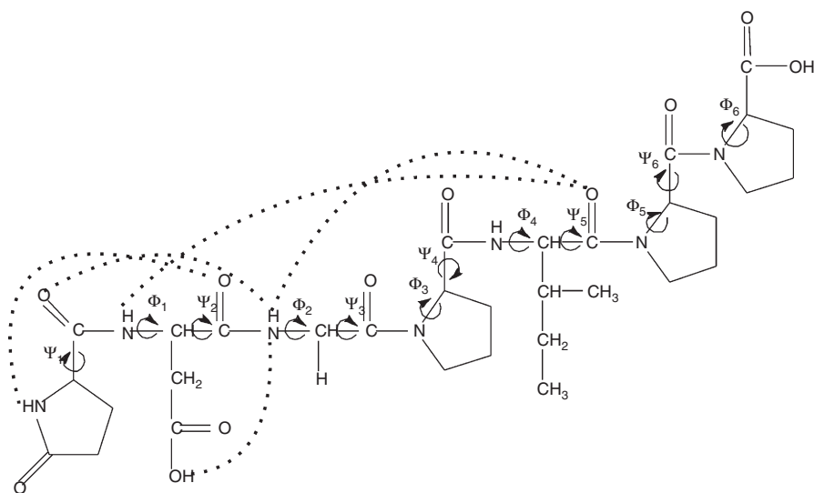
Figure 5.5 The chemical structure of BPP7a, [ p -Glu 1 Asp 2 Gly 3 Pro 4 Ile 5 Pro 6 Pro 7 ]. For clarity, dihedral angles and intramolecular HBs are indicated.
