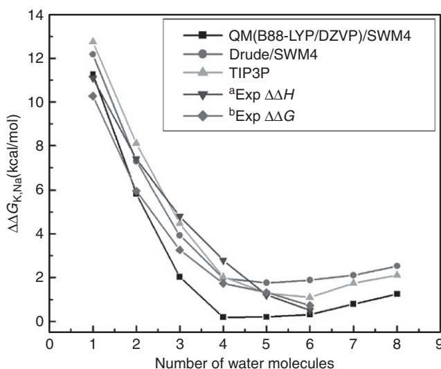
Figure 10.4 Relative (to the bulk) free energy of selectivity for Na^+/K^+ in water clusters as a function of cluster size. Experimental information is taken from a Ref. [192] and b Ref. [193].
