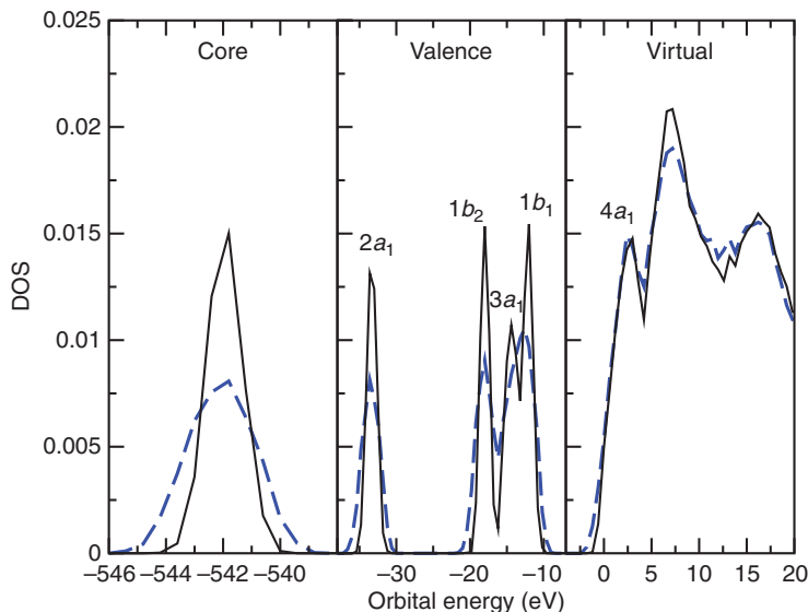
Figure 4.8 Average electronic DOS of liquid water at T = 298 K from sequential Monte Carlo/DFT calculations. The average DOS was calculated over 50 configurations. The QM system includes 30 water molecules. The surrounding water molecules (200) are represented by TIP5P charges. Results for a nonembedded QM system are also shown (dashed lines). Reprinted with permission from J. Chem. Phys. 123 (2005), 054510, Copyright 2005, AIP.
