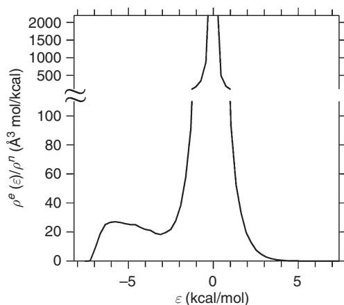
Figure 9.5 The distribution function of the pair interaction energy \varepsilon of water at 1\text{ g/cm}^3 and 25^\circ\text{C} . \rho^n is the (number) density in the system.
