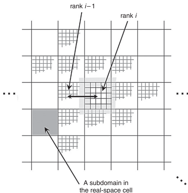
Figure 9.1 Illustration of the division of the real-space cell in the parallel implementation. Each core processor (rank) is charged with the computation for a subdomain. The area of which data must be communicated is colored in the figure. The line with arrows at both ends represents the data exchange between neighboring cores [rank i and rank (i - 1) ].
