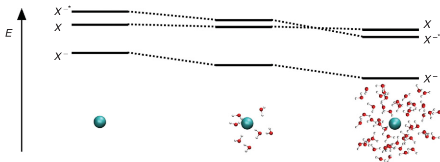
Figure 4.12 Energy diagram for three electronic states of the halide—ground state ( X^- ), excited state ( X^{*-} ), and ionized state ( X ). The ordering is given according to the environment (from left to right, gas, cluster, and aqueous solution).
