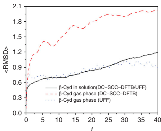
Figure 5.2 Root-mean-square deviation, \langle RMSD \rangle , see Eq. (38), of the coordinates between two snapshots of an MD trajectory (in Å) (gas phase in dashed line) against simulation time t (in ps). The simulation in solution is given as black solid line, the DFTB and MM gas phase simulation as dashed line and dotted line, respectively. Please refer online version for color image.
