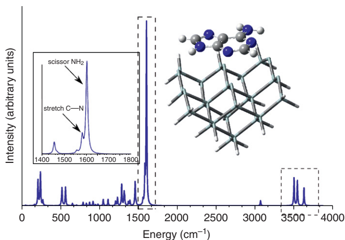
Figure 2.8 IR spectrum of adenine@Si 28 with five most intense bands included in anharmonic computation.
