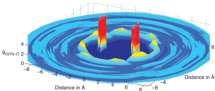
Figure 7.13 Two-dimensional U(VI)-O pair correlation plot. The second shell of the U(VI) atom as well as the first shell of the oxo atoms can be easily identified, which is not possible by an unspecific full sphere radial distribution function.
