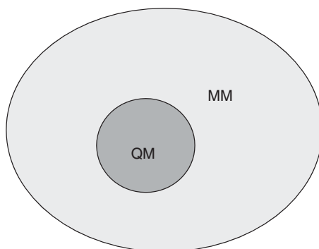
Figure 1.1 The combined QM/MM model.
