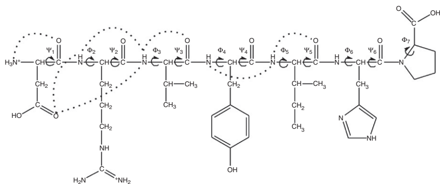
Figure 5.8 The chemical structure of angiotensin-(1–7), [AspArgValTyrIleHisPro]. Dashed lines show the intramolecular HBs present during the simulation of Ang-(1–7) in aqueous solution. See text for detail.
