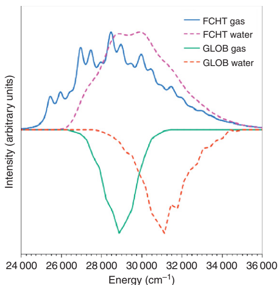
Figure 2.3 UV spectra of n \rightarrow \pi^* electronic transition of acrolein. Upper panel, time-independent approach, spectra computed with FC-HT approximation, gas phase (solid line), and water solution described by the CPCM model (dashed line). Lower panel, time-dependent approach: spectra obtained from MD simulations with the GLOB model, gas-phase spectrum (solid line), and aqueous solution (dashed line). Please refer online version for color image.
