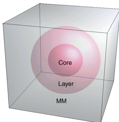
Figure 7.1 Scheme of a QMCF simulation: the chemical most relevant region is treated by quantum mechanics (QM), the remaining part by molecular mechanics (MM). For coupling purposes the QM region is again separated into two zones, namely, the “QM core” and the “solvation layer.”
