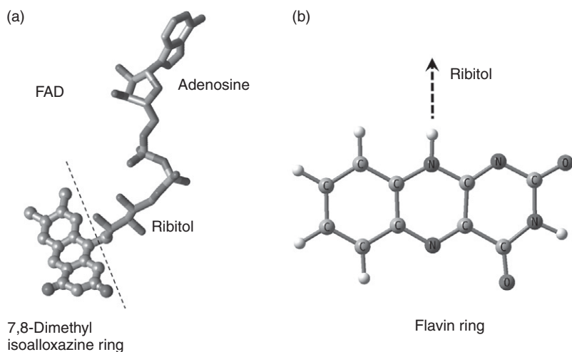
Figure 9.11 Ball and stick illustrations for the (a) flavin adenine dinucleotide (FAD) and the (b) flavin ring. The two methyl groups in the 7,8-dimethyl isoalloxazine ring in FAD are replaced by hydrogen atoms in the construction of the flavin ring to reduce the computational cost in the present calculation.
