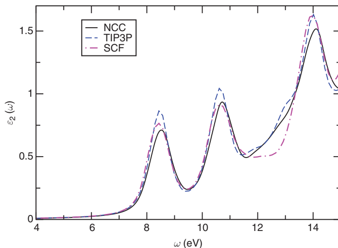
Figure 4.6 Dependence of the imaginary part of the dielectric constant of liquid water [ \epsilon_2(\omega) ] on the choice of the charge background. Results for TIP3P, NCC, and SCF charges are from TDDFT BH and HLYP/dapvdz calculations with N_w = 1 .
