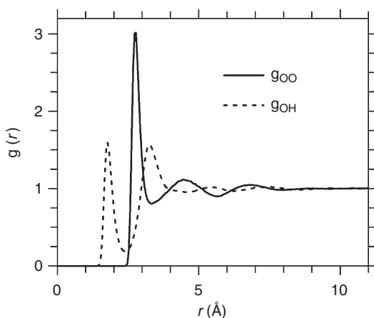
Figure 9.4 O—O and O—H radial distribution functions of water at 1\text{ g/cm}^3 and 25^\circ\text{C} .
