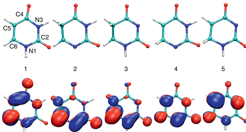
Figure 2.7 Optimized structures and corresponding single occupied molecular orbitals of five tautomers of the uracil radical anion, including the canonical form, obtained at B3LYP/N07D and C-PCM level.
