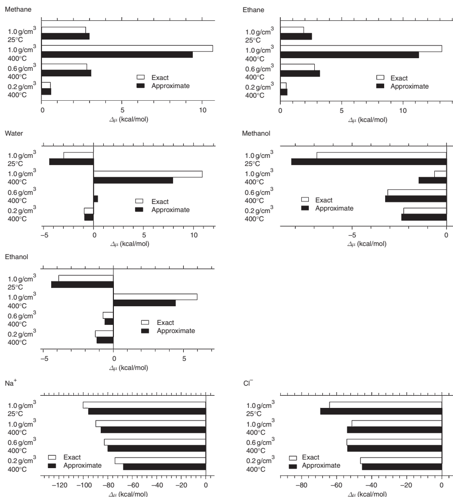
Figure 9.6 The solvation free energy \Delta\mu calculated by the approximate method of energy representation and the exact, free-energy perturbation method. The thermodynamic state is specified by the solvent density and temperature.
