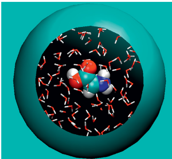
Figure 2.1 Graphical representation of a solute–solvent system simulated using the GLOB model: the explicit system is embedded into a spherical cavity of a dielectric continuum.
