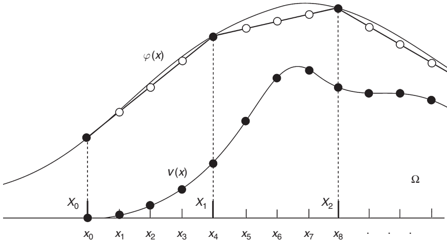
Figure 9.2 Schematic for the one-dimensional double grids in the atomic core region \Omega . \varphi(x) and v(x) are the wave function and the nonlocal pseudopotential, respectively. Arrays \{X_i\} and \{x_i\} denote the coarse and dense grids, respectively. The values on the black points are to be evaluated explicitly, while those on the white ones are obtained by an interpolation.
