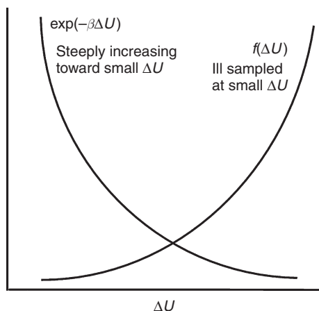
Figure 9.3 A schematic distribution of \Delta U value in the particle insertion method.
