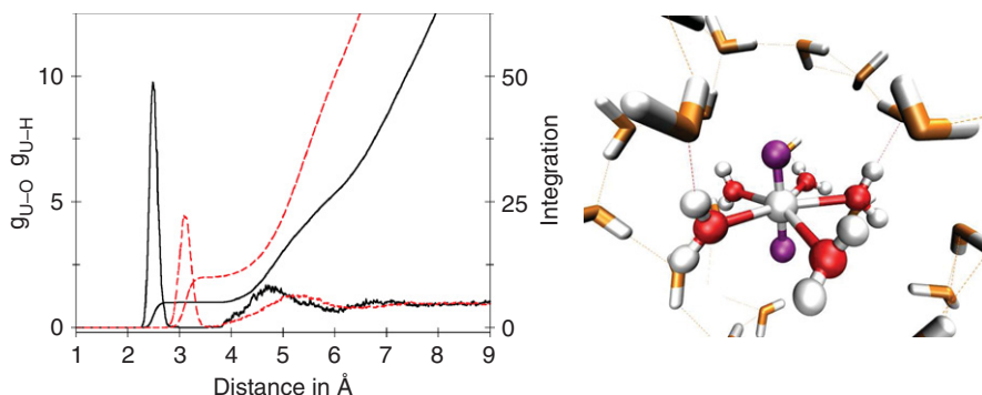
Figure 7.11 U—O (solid line) and U—H (dashed line) radial distribution functions (left side). Snapshot of the simulation (right side).
