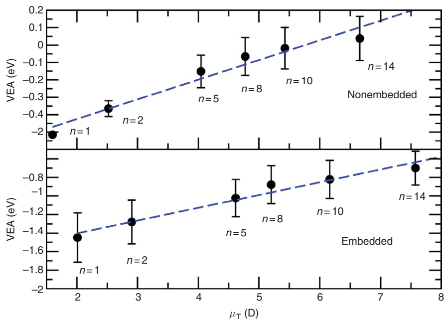
Figure 4.11 Average VEA (in eV) versus average total dipole moment ( \mu_T in D) of ammonia clusters. Dashed lines are fitting to raw data with correlation coefficients r = 0.977 (nonembedded) and r = 0.983 (embedded clusters). Reprinted with permission from J. Chem. Phys. 128 (2008) 014506, Copyright 2008, AIP.
