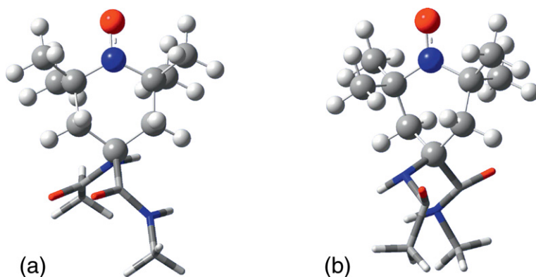
Figure 2.9 The chair (a) and twisted (b) structures of TOAC. The QM part is presented as balls and sticks, while the tubes correspond to the MM part.
