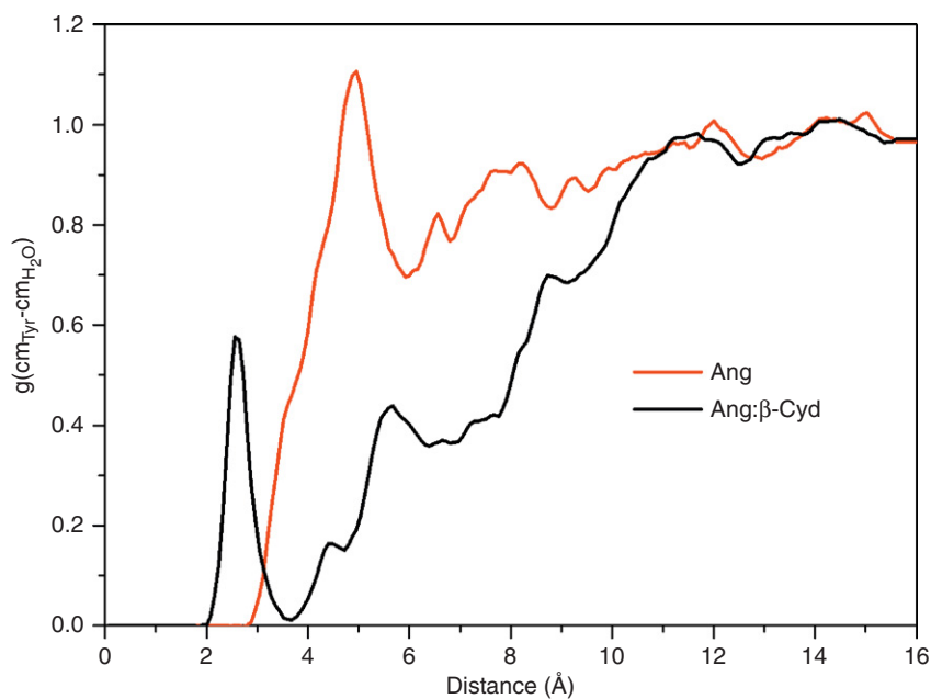
Figure 5.13 Radial distribution functions of the water around the tyrosine residue in the Ang-(1-7).
