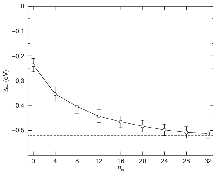
Figure 4.15 Solvatochromic shift \Delta\omega of the \pi \rightarrow \pi^* excitation of the acrolein molecule (in eV), embedded in a solvent sphere with a 20 \text{ \AA} radius. The shift is computed with use of Eq. (20), and shown as a function of the number of water molecules treated quantum mechanically ( n_w ).
