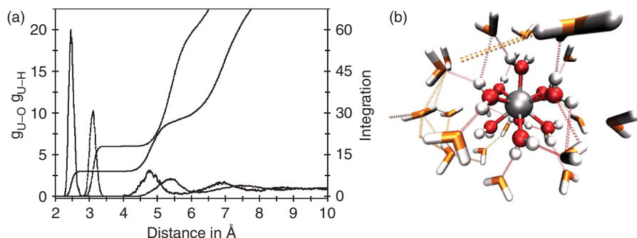
Figure 7.4 (a) Ion–oxygen (solid line) and ion–hydrogen (dashed line) radial distribution function obtained from a QMCF MD simulation of U(IV) in aqueous solution. (b) Snapshot of the simulation.
