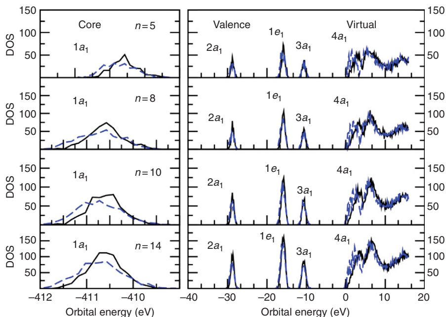
Figure 4.10 Electronic DOS of ammonia clusters ( n = 5, 8, 10 , and 14 ) in the presence (solid line) and absence (dashed line) of an embedding background. Reprinted with permission from J. Chem. Phys. 128 (2008) 014506, Copyright 2008, AIP.
