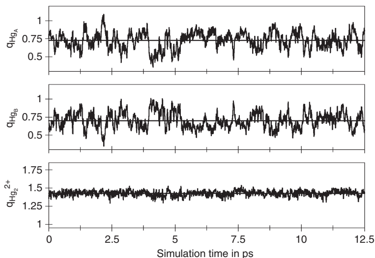
Figure 7.8 Partial charges of the individual Hg(I) atoms and the respective sum (same scaling for all plots).
