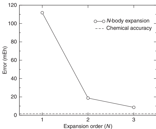
Figure 4.1 Error in the total energy (in milliHartree) of a N -body expansion of a water octamer. The results are given for HF/cc-pVDZ calculations.
