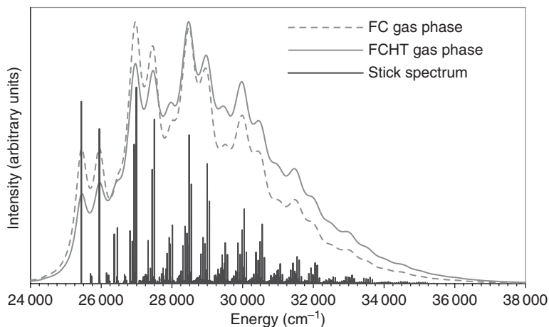
Figure 2.4 OPA spectra of n \rightarrow \pi^* electronic transition of acrolein computed by time-independent approach. Gas-phase spectra computed with FC approximation (dashed line) and the FC–HT approximation (solid line), convoluted by homogeneous broadening with FWHM of 400 cm -1 . The FC–HT stick spectrum is also shown. Please refer online version for color image.
