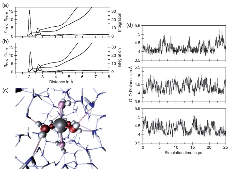
Figure 7.5 Ion–oxygen (solid line) and ion–hydrogen (dashed line) radial distribution function obtained from a QMCF MD simulation of (a) Pd(II) and (b) Pt(II) in aqueous solution. (b) Snapshot of the Pt(II) simulation. (c) O–O distances of water molecules in trans-position observed in the course of a QMCF MD simulation of hydrated Cu(II).
