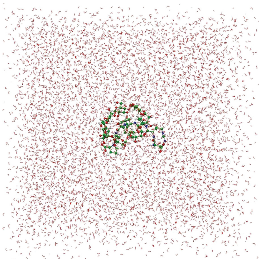
Figure 5.11 Box of water used to simulate Ang-(1-7): \beta -Cyd in solution.
