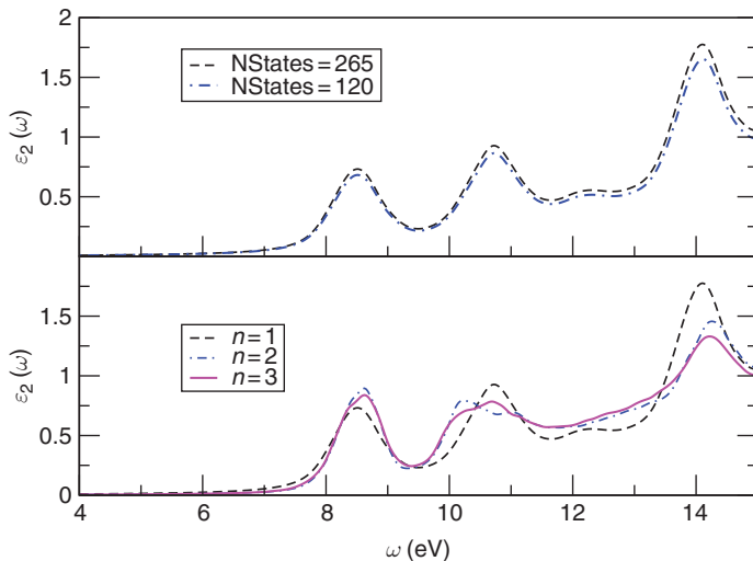
Figure 4.5 Bottom: dependence of the imaginary part of the dielectric constant of liquid water [ \epsilon_2(\omega) ] on the number of water molecules in the quantum system. Results are from TDDFT BH and HLYP/dapvdz calculations; top: behavior of \epsilon_2(\omega) with the number of states (NStates) included in the SOS for a system with N_w = 1 . Reprinted with permission from J. Chem. Phys. 130 (2009) 014505. Copyright 2009, AIP.
