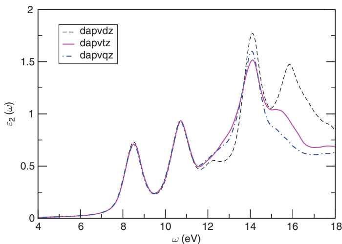
Figure 4.4 Basis set dependence of the imaginary part of the dielectric constant of liquid water [ \epsilon_2(\omega) ]. Calculations were carried out with the BH and HLYP functional and a single water molecule in the quantum system. Results are shown for dapvdz, dapvtz, and dapvqz basis sets.
