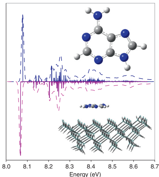
Figure 2.10 Comparison between the theoretical photoionization spectra in gas phase of isolated adenine (upper panel) and adenine adsorbed on a Si(100) surface (lower panel). The spectra in an energy range from 8.0 to 8.7 eV are calculated with FC approximation and with FWHM = 100 cm -1 ; the stick bands show the most important transitions. Please refer online version for color image.
